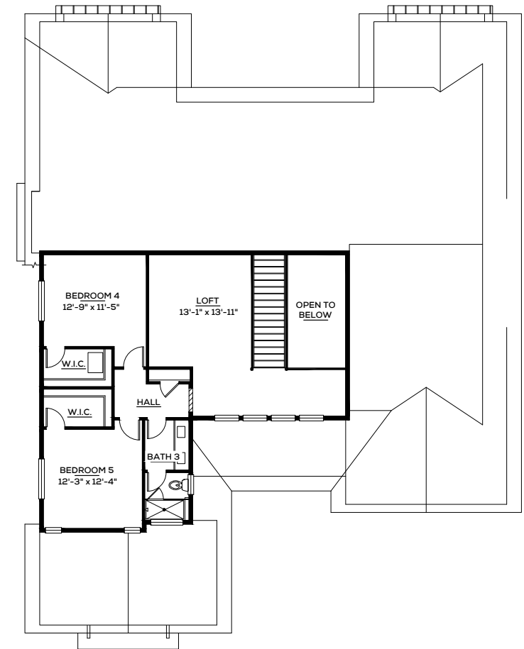
Opt. Upper Level - Plan A
