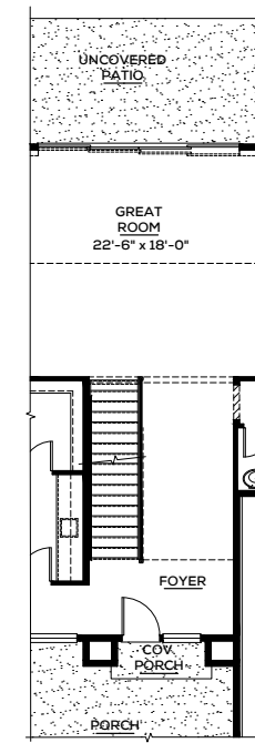
Plan A - Main Level with Opt. Upper Level
