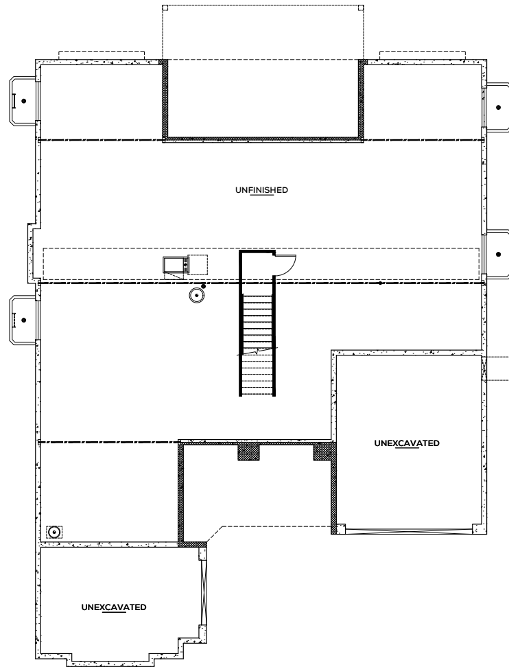
Plan B Partial Unfinished Lower Level Floor Plan (2,488 sq.ft.)
