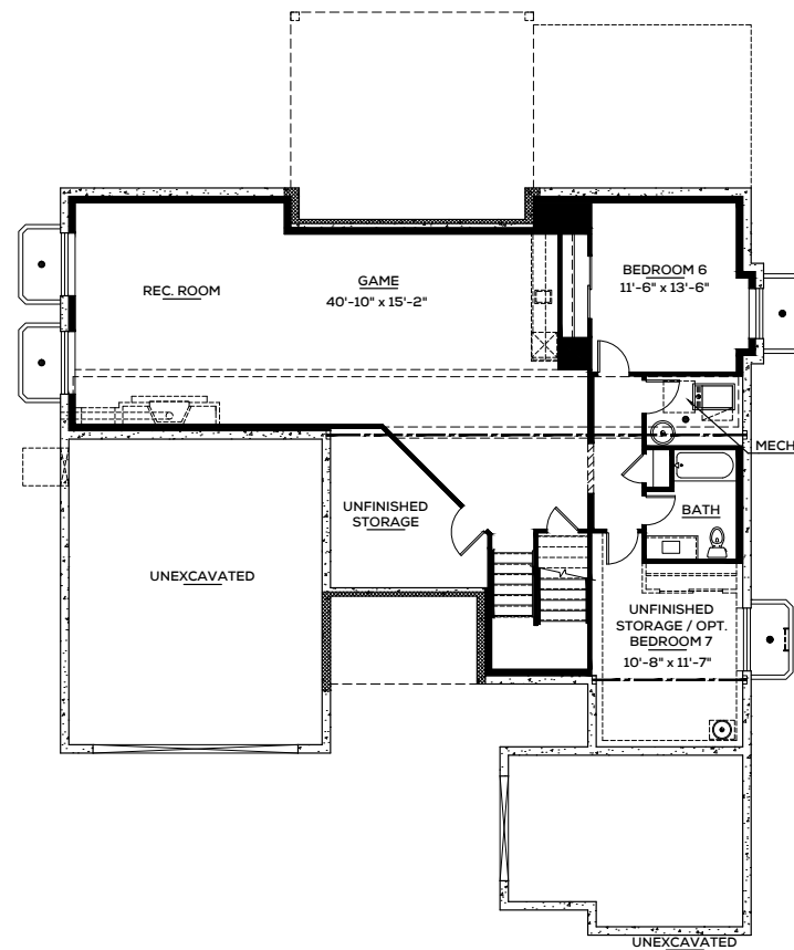
Plan B - Lower Level Opt. Finished Basement
