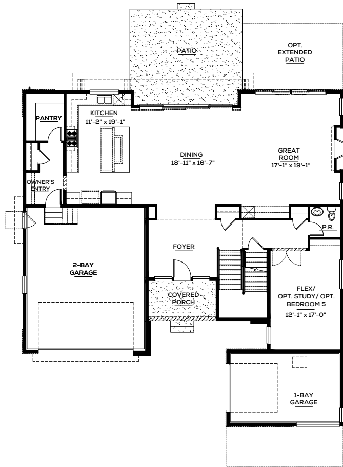
Plan B Main Level Floor Plan
