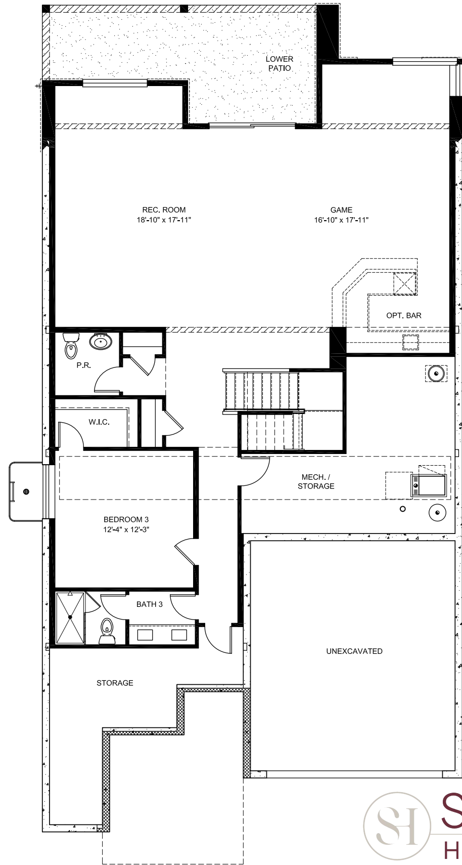
Lower Level Floor Plan
