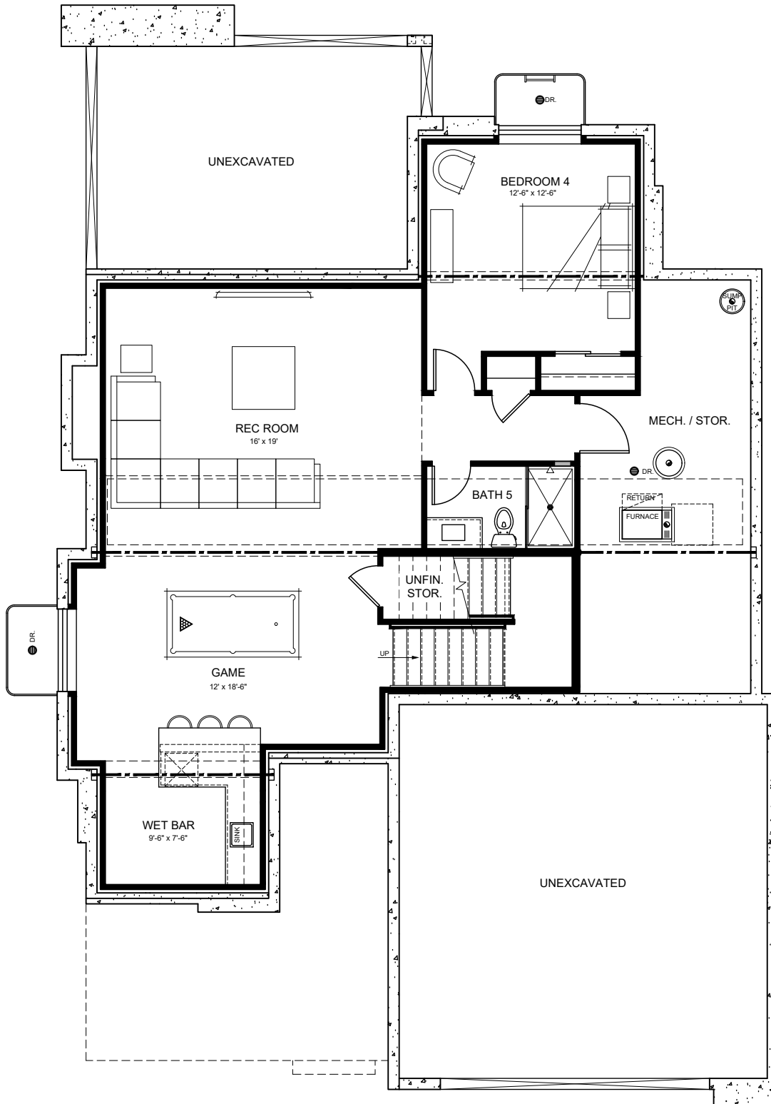
LOWER LEVEL FLOOR PLAN 954 sqft
